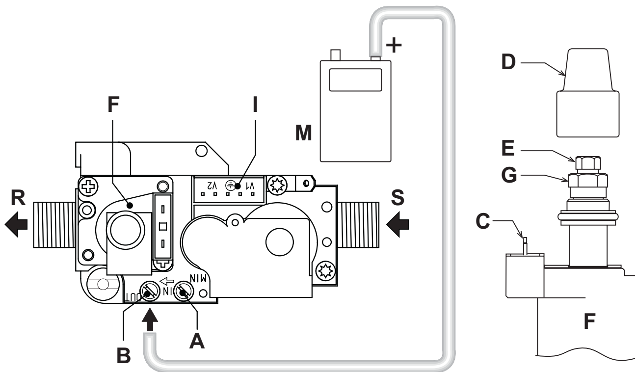
fig. 23 - Valvola gas
